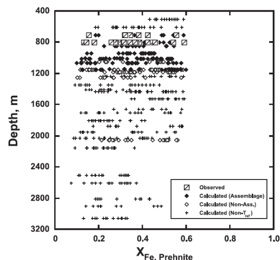
Figure 5: Calculated (diamonds) and measured (squares) X_{\text{Fe,Prehnite}} values as a function of depth in wells RN-9, RN-10 and RN-17. The measured values are from RN-17, but the calculated values have been derived from epidote compositions in RN-9, RN-10 and RN-17 using equations 16 and 20. The solid diamonds (assemblage) are computed from measured compositions of epidotes at depths where prehnite, quartz and calcite are also found in the drill cuttings, and the open diamonds (non-assemblage) are from depths where prehnite and/or calcite are absent from the cuttings. Only samples found in cuttings at depths where reference temperatures range between 274 and 310°C are denoted as “assemblage” or “non-assemblage.” All other values are labeled as “Non- T_{\text{ref}} .”
