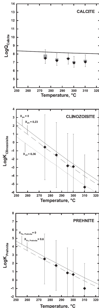
Figure 9: Saturation conditions for calcite (a), epidote (b) and prehnite (c) in the Reykjanes geothermal system based on the distribution of aqueous species for measured geothermal. Solid lines represent values of the equilibrium constant as a function of temperature for reactions (20), (21) and (22) and the symbols denote values of the ion activity products for these reactions (Eqn. 23). Error bars denote \pm 0.3 pH units. Broken lines in diagrams b and c denote isopleths for the noted compositions of epidote and prehnite solid solutions
