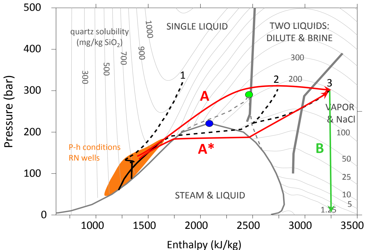
Figure 5: Phase diagram for H 2 O shown in Figure 2, with added potential fluid recharge paths (A and A*) and production path (B) of scenario 3 fluid.
