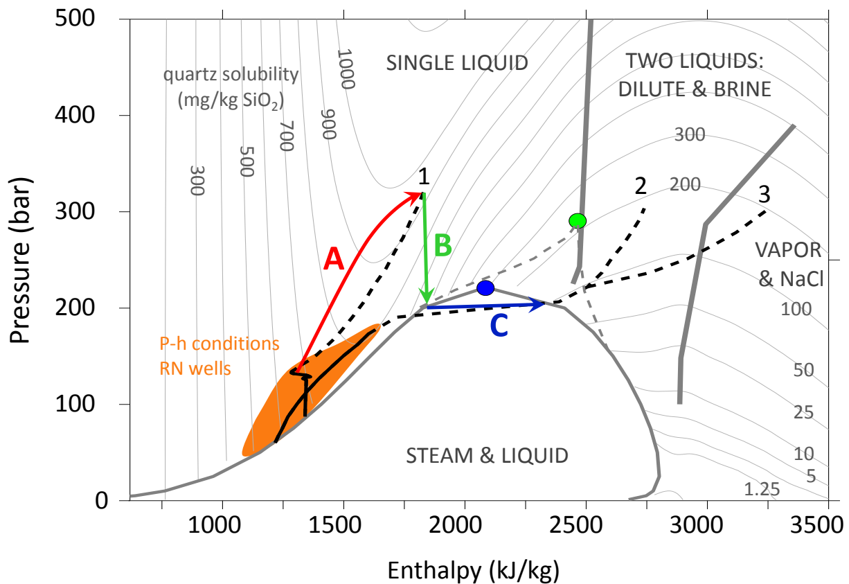
Figure 3: Phase diagram for H 2 O shown in Figure 2, with added potential fluid recharge path (A) and production paths (B and C) of scenario 1 fluid.
